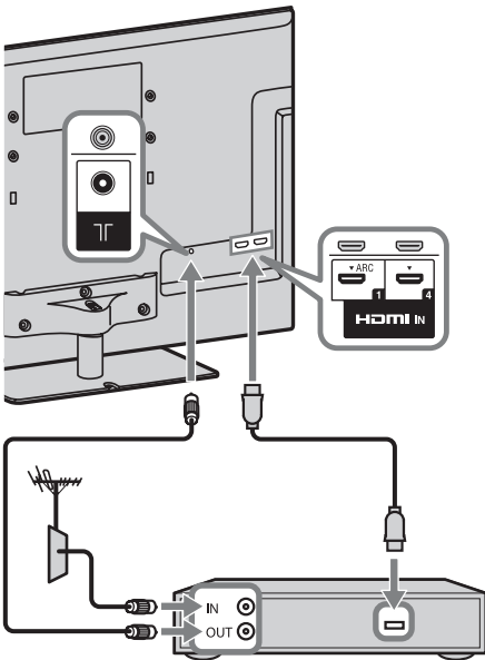
Set Top Box/recorder (e.g. DVD recorder)
