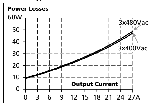
Fig. 11-2 Losses vs. output current at 36V, typ.
