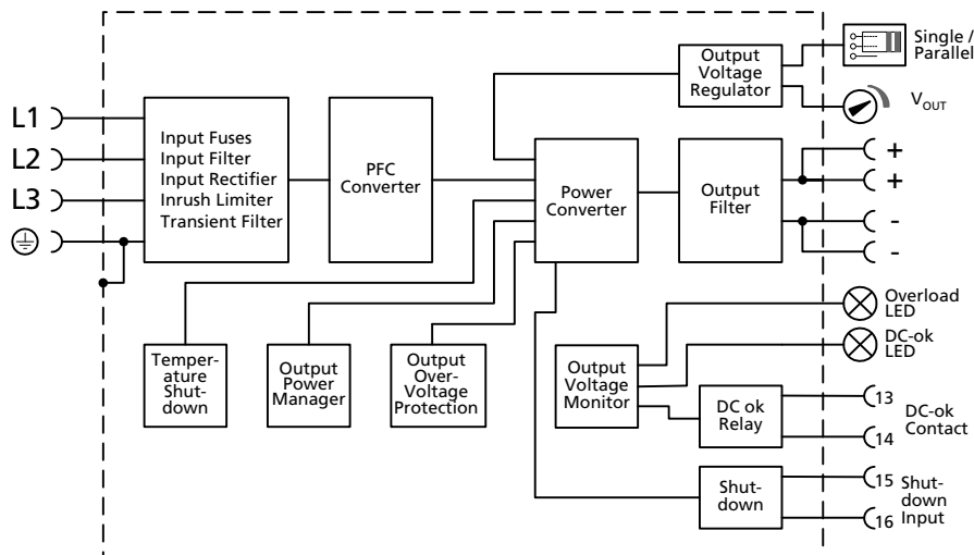
Fig. 13-1 Functional diagram
