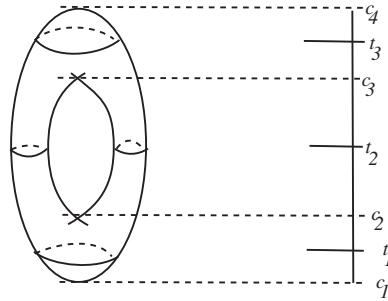
Fig. 2.13. Slicing a manifold by a Morse function.
