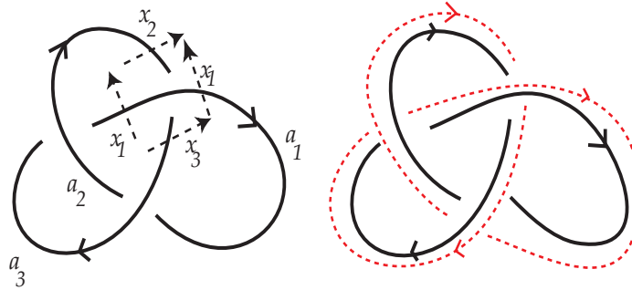
Fig. 2.2. The (left-handed) trefoil knot and its blackboard parallel.
