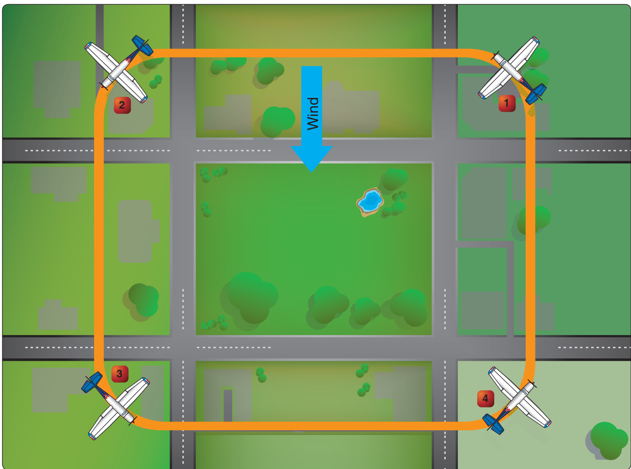
FIGURE 62.—Rectangular Course.
