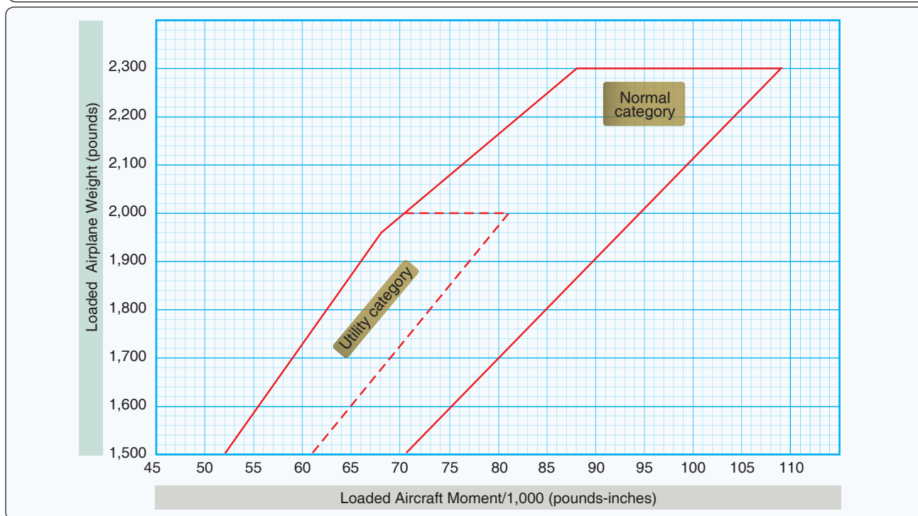
FIGURE 34.—Airplane Weight and Balance Graphs.
