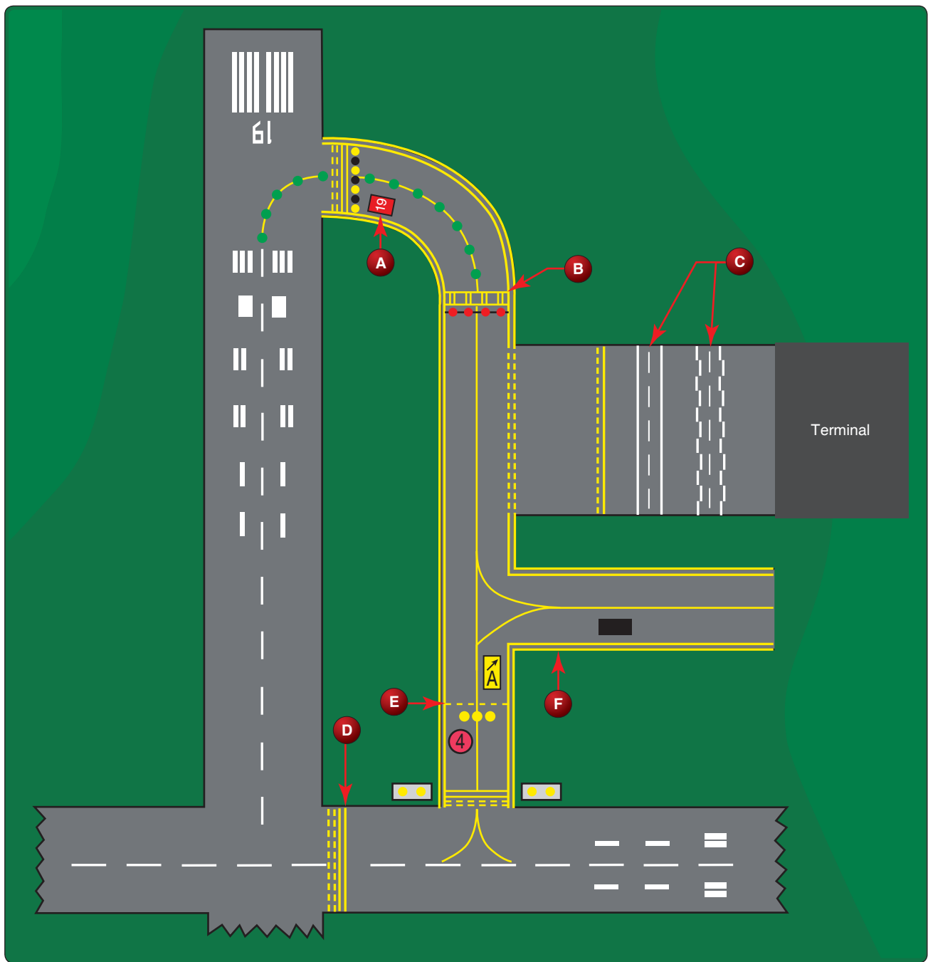
FIGURE 64.—Airport Markings.
